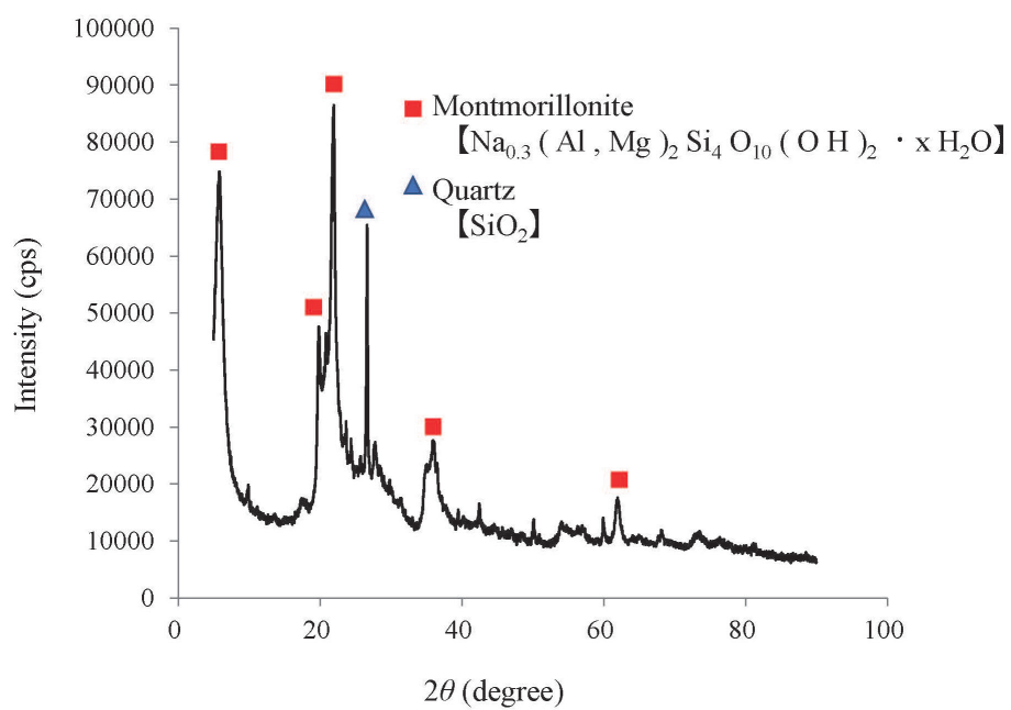
Fig. S3. XRD Pattern of the AC
