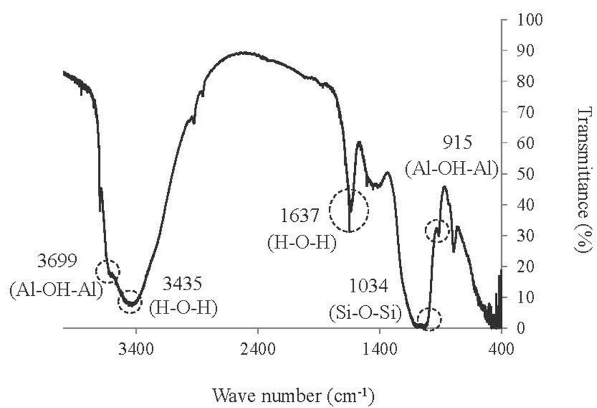
Fig. S2. FT-IR of the AC
