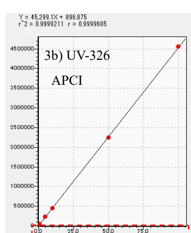
Fig. S1 Comparison of calibration curves for ESI and APCI in this study
