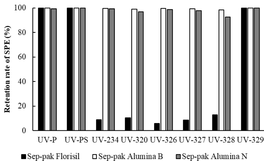
Fig. S2 Evaluation of BUVs retention on different solid-phase extraction cartridges based on elution with acetone:hexane (1:9, v/v).
