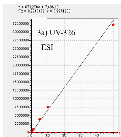
Fig. S1 Comparison of calibration curves for ESI and APCI in this study
